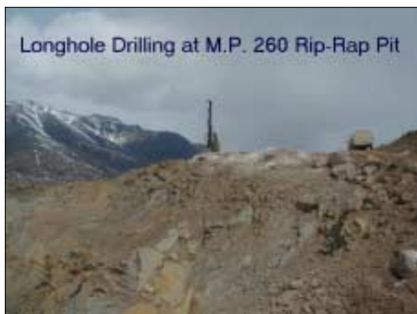
Figure 21. Longhole drilling at the DOTPF rip-rap pit at mile 260 of the Dalton Highway. Photo provided by Bill Cole, Alaska Department of Transportation & Public Facilities (DOTPF).
